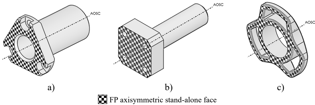
Figure 47. Examples of local FP symmetry detection
