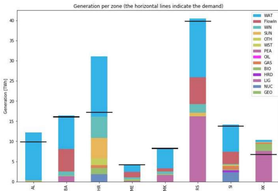
Figure 21 Generation of electricity per zone in case of high cost of CO 2
