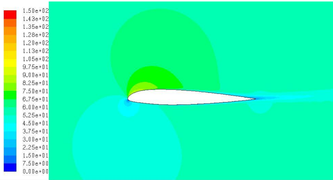
Contours of Velocity Magnitude (m/s)
