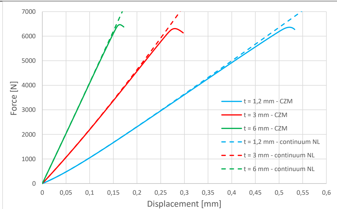
Figure 47. Force-displacement curve comparison between CZM and continuum models for different adherend thicknesses
