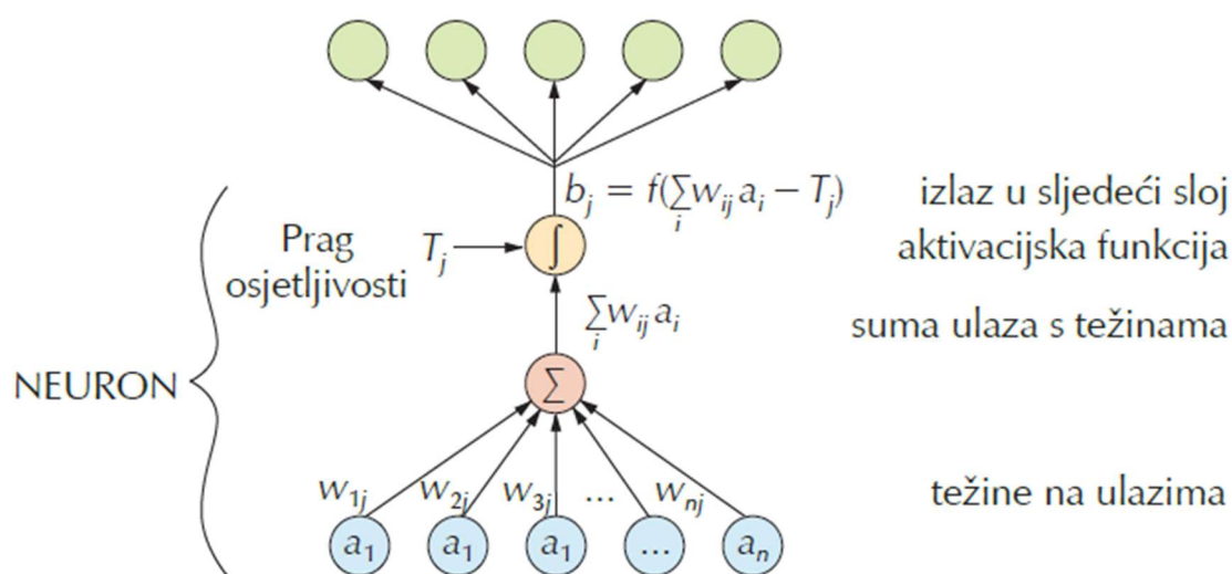
Slika 4. Model perceptrona
