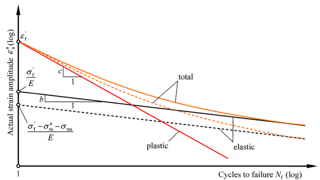
Fig. 6. Schematic representation of strain-life approach with Morrow's mean stress correction.
