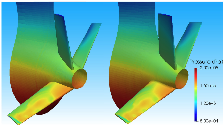
Fig. 13. Hydrodynamic pressure transfer on the FEM-CFD interface surface. Fluid mesh (left), structural mesh (right).
