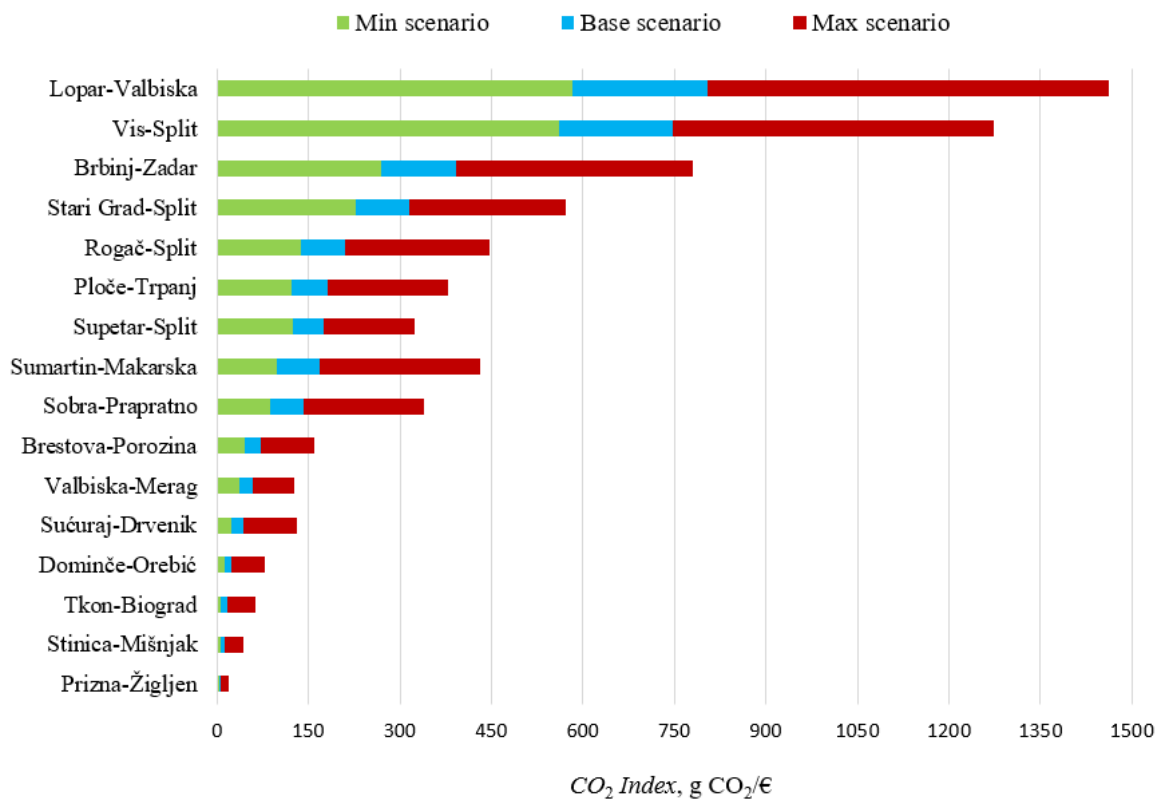
Figure 9. Sensitivity analysis
