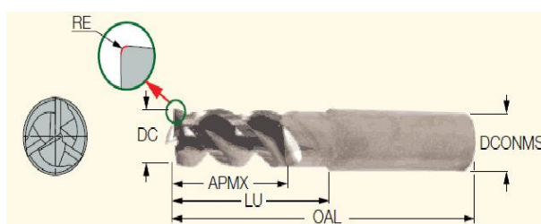
Slika 39. ECA-H3 12-24/36C12CF-R02C [10]
