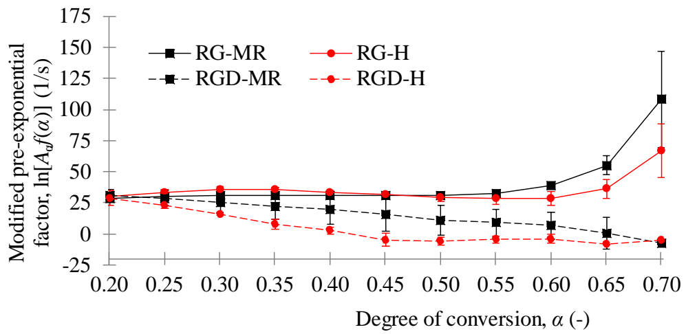
Figure 2 Distribution of E_\alpha and \ln[A_d f(\alpha)] with the degree of conversion by means of FR model
