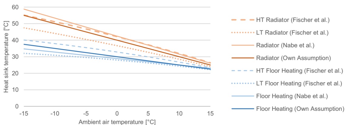
Figure 6 Space heating temperature regimes in different systems [13]
