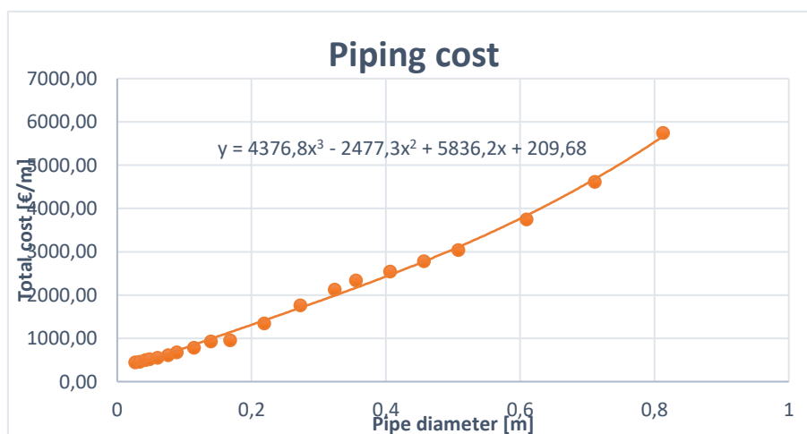
Figure 34 Pipe total cost as a diameter function [36]
