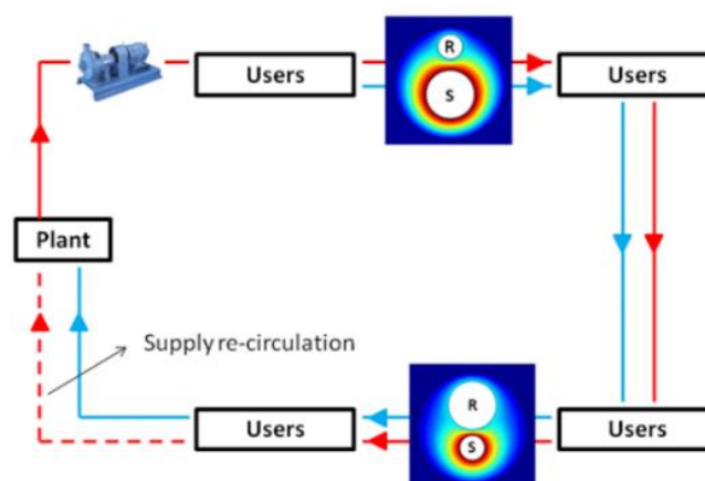
Figure 5 Double pipe network [4]
