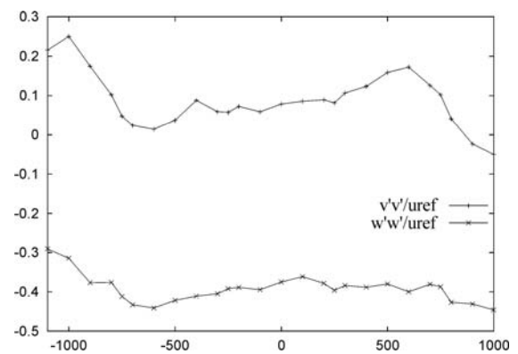
\sqrt{v'v'}/u_{ref} ; \sqrt{w'w'}/u_{ref}
