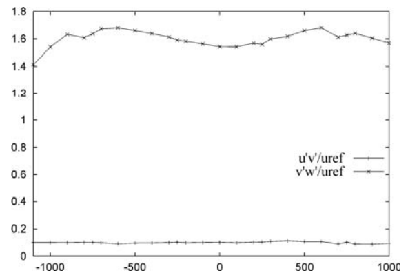
\sqrt{u'v'}/u_{ref}^2 ; \sqrt{v'w'}/u_{ref}^2
