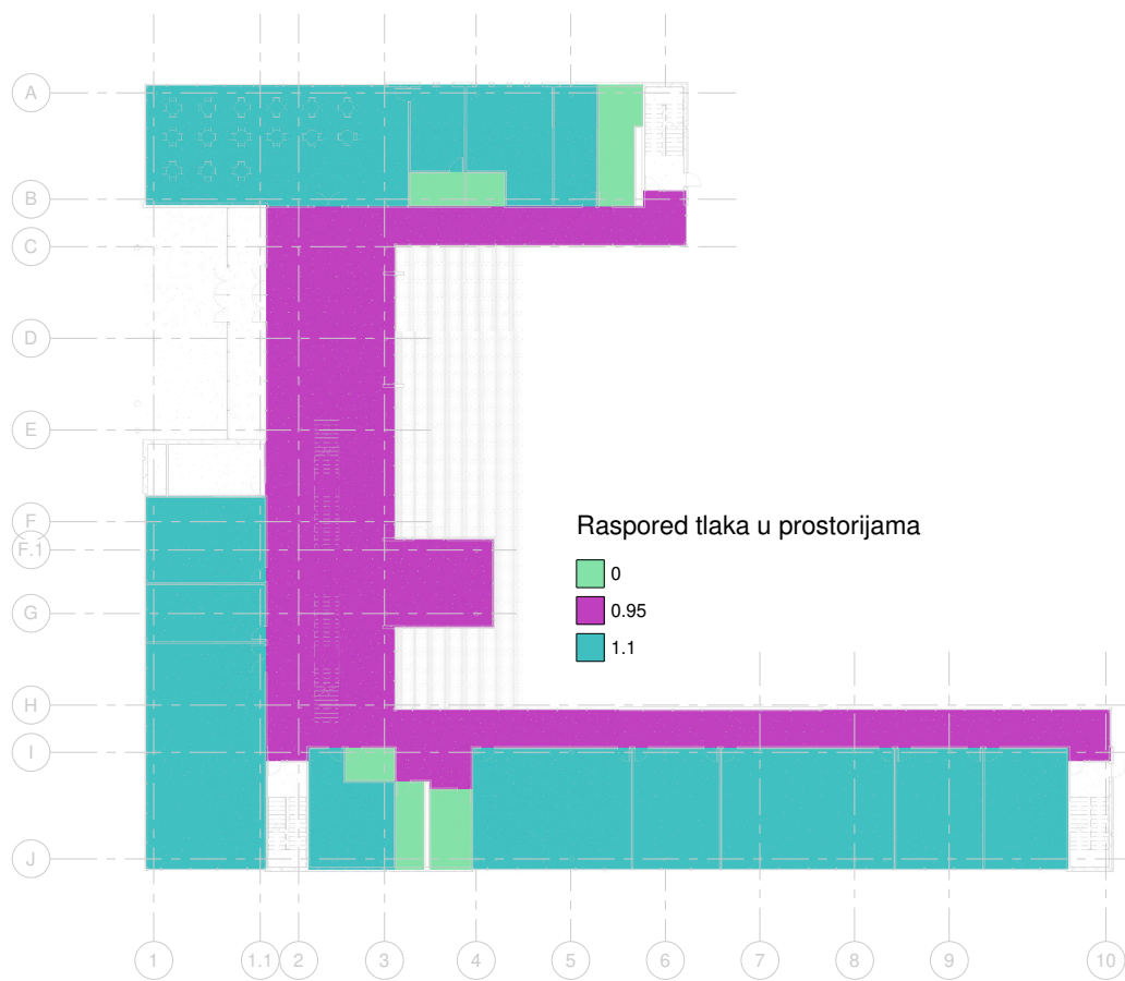
2 Raspored potlaka i pretlaka 1 : 200
