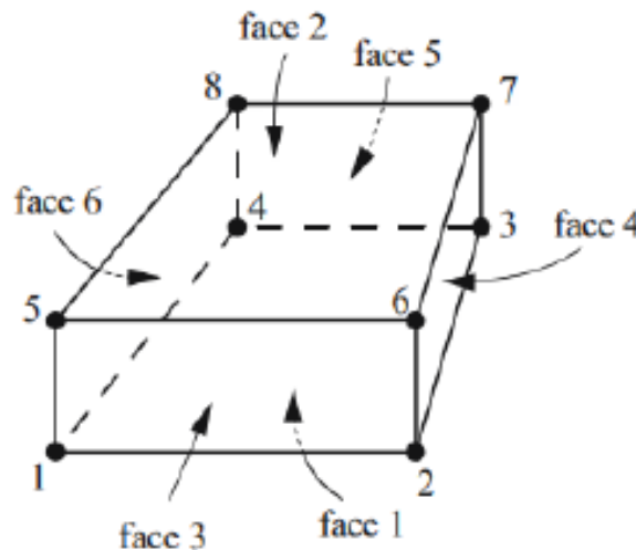
Figure 3.10: C3D8R element [27]
