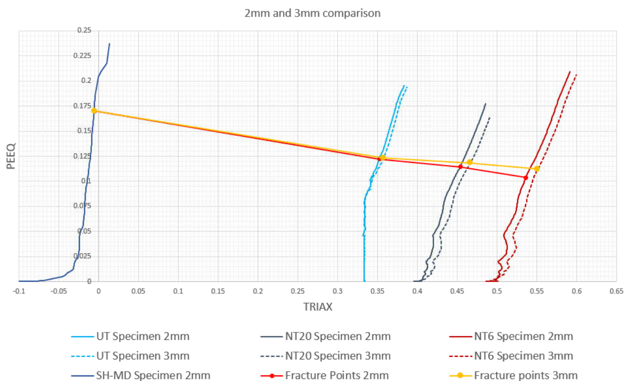
Figure 4.3: Strain paths of 2 and 3 mm specimens
