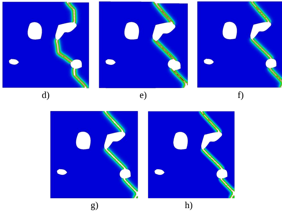
Fig. 5.15. Monotonic loading. Crack paths obtained on specimen S with N2 with a) G_c = 0.001 N/mm, b) G_c = 0.002 N/mm, c) G_c = 0.005 N/mm d) G_c = 0.01 N/mm, e) G_c = 0.1 N/mm, f) G_c = 0.25 N/mm, g) G_c = 0.45 N/mm, and h) G_c = 0.74 N/mm
