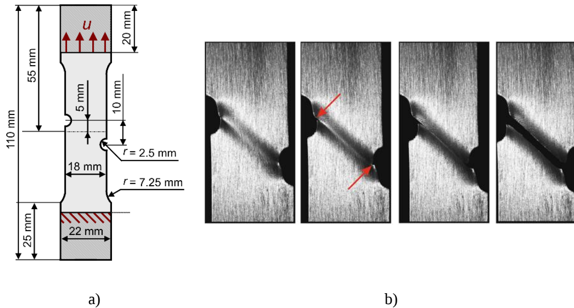
Fig. 4.23. Asymmetrically notched specimen. a) Geometry and boundary conditions, b) Experimental results [105]
