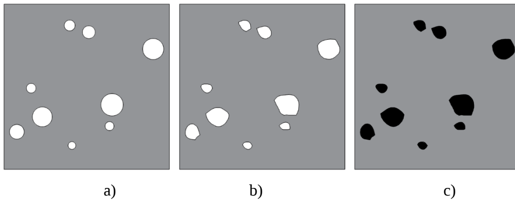
Fig. 5.3. Schematic representation of nodule modelling options a) circular holes (N1), b) holes of corresponding to the nodule shape (N2), c) nodules as inclusions of corresponding shape (N3)
