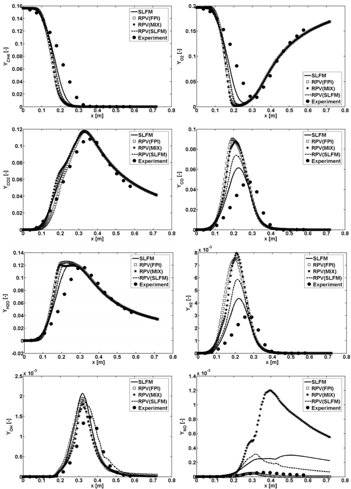
Figure 59 – Axial profiles (centreline) of mean species mass fractions (methane flame)
