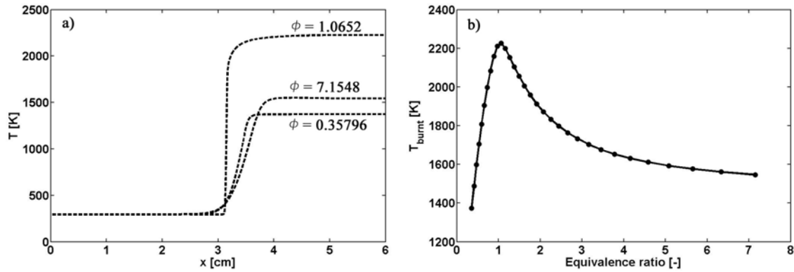
Figure 4 – Adiabatic temperature profiles from the premixed flamelet database (diluted methane (25% CH 4 , 75% air – by volume)/air): a) T-x plots; b) T burnt - \phi plot
