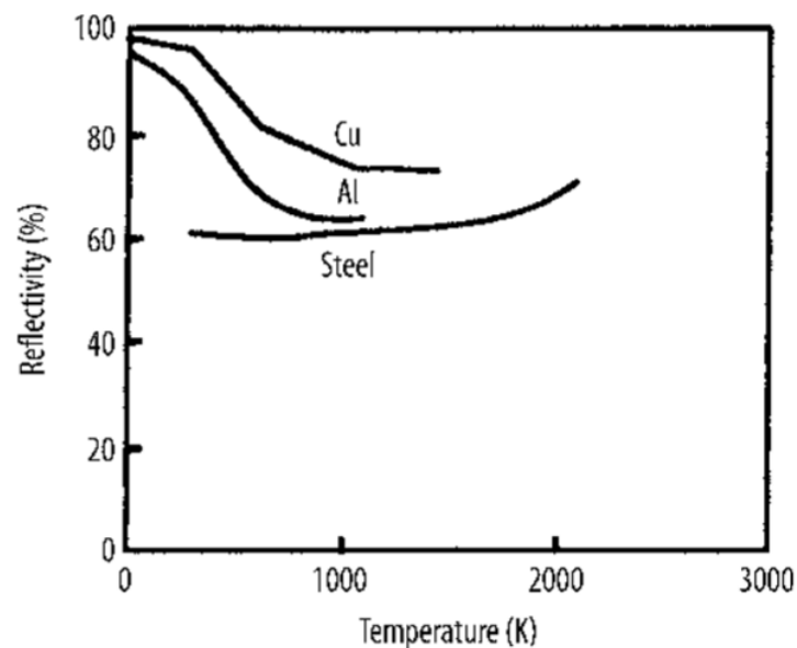
Figure 8 Reflectivity-temperature dependence of a 1,06 μm radiation [1]
