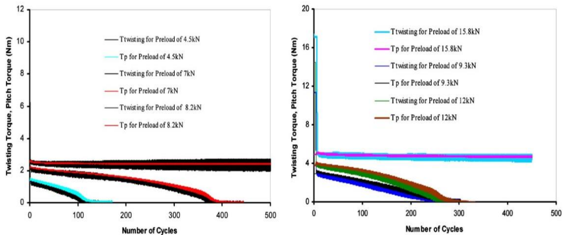
Figure 15. The Twisting Torque variation of the Strain Gauged Bolt under Displacement Amplitude 0,3556 mm (Left) and under Displacement Amplitude 0,61 mm (Right) [17]
