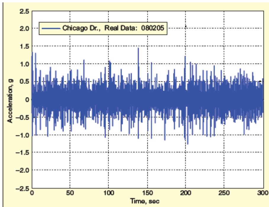
Figure 24. Random Acceleration Time History [26]
