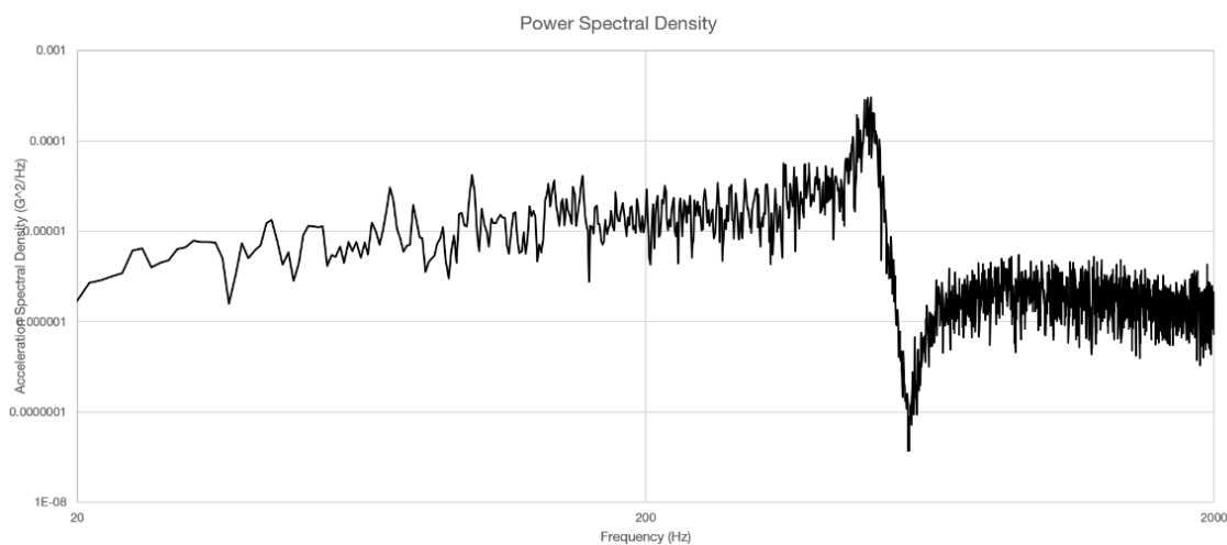
Figure 31. PSD Curve [30]
