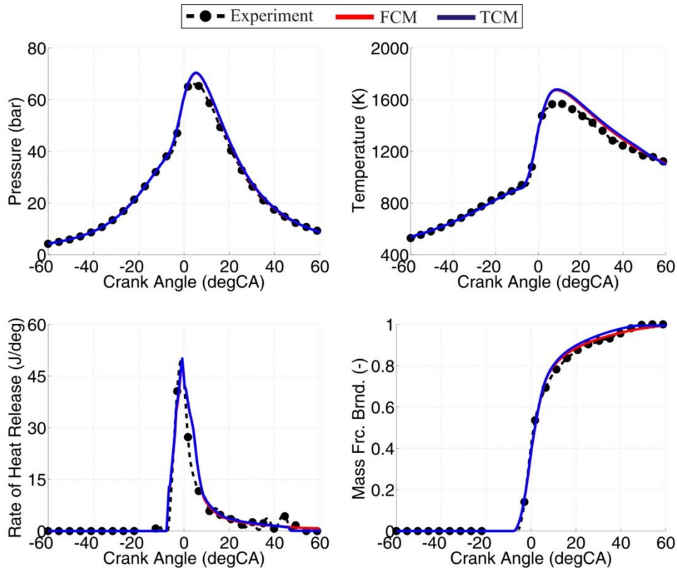
Figure 172. Comparison between the measured and simulated in-cylinder pressure, temperature, ROHR and MFB traces for OP2 at 1800 rpm
