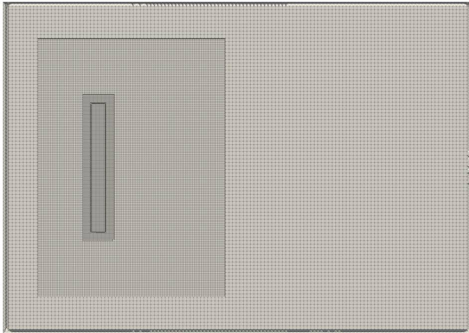
Figure 3.3.1: Intercooler: volume mesh.
