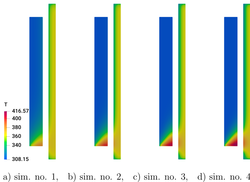
Figure 3.4.7: Simultaneous operation, XZ cross section of intercooler and radiator: air temperature.
