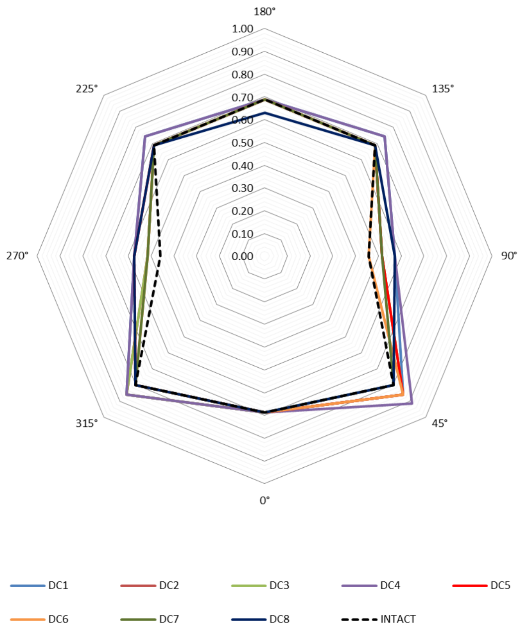
Figure 32 Maximum pitch motion for different wave heading angles.
