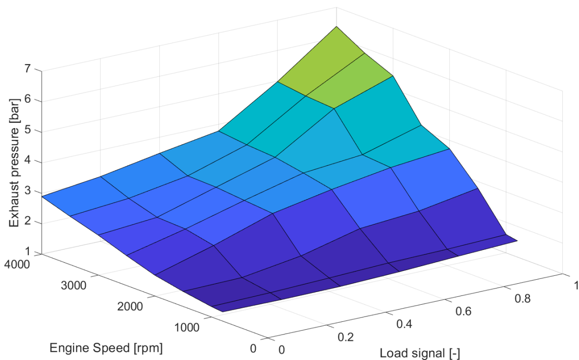
Figure 13. CI engine exhaust pressure look-up table, Appendix A, Engine 2
