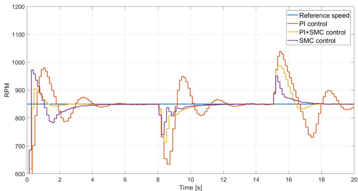
Figure 47. ISC response of Engine 4, data from Appendix A, various control systems
