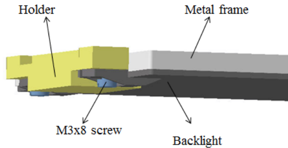
Figure 54. CAD model holder with backlight
