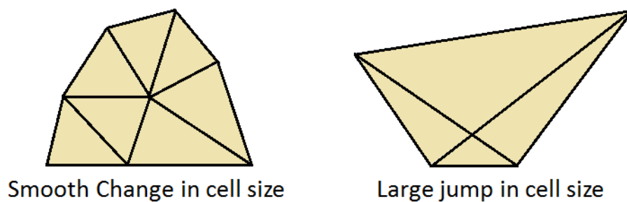
Figure 14. Change in size mesh quality
