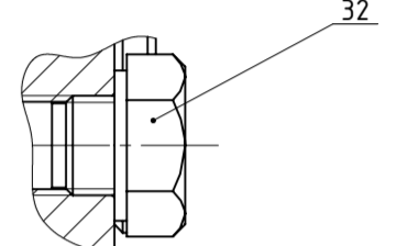
Detailj H M1:1
