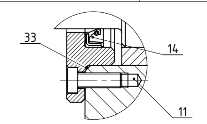
Detailj A M1:1
