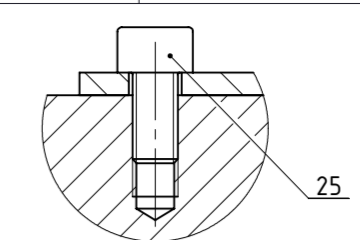
Detailj C M1:1
