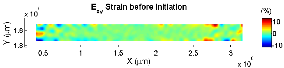
Figure 4.41: Computed E_{xy} strain before crack initiation - \gamma = 1.8 sample
