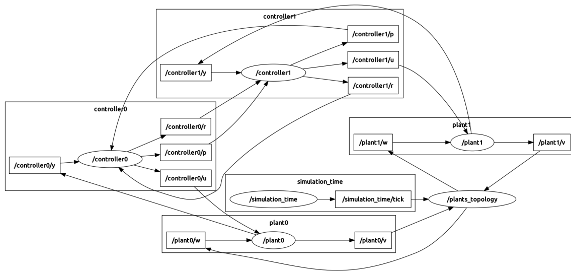
Figure 5.12: Runtime graph
