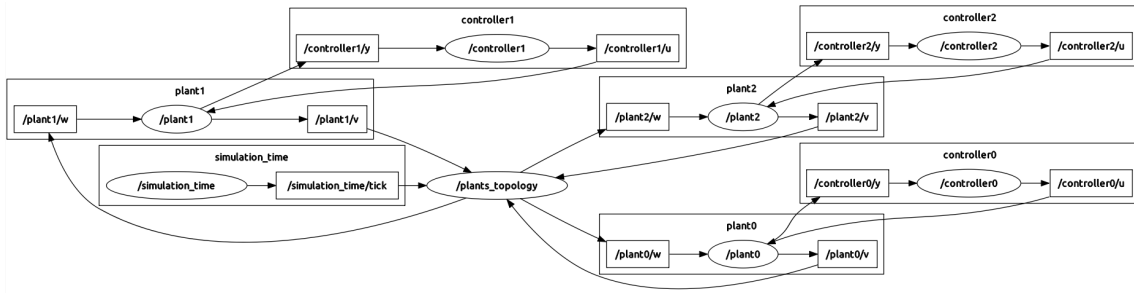
Figure 5.4: Runtime graph
