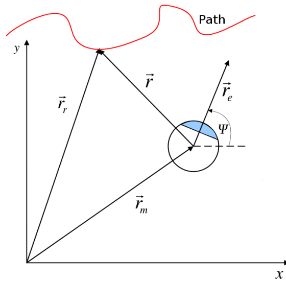
Figure 5.8: Vectors describing the boat's position
