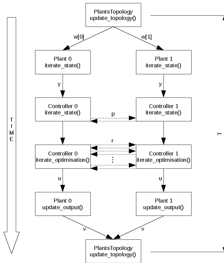
Figure 4.10: Execution flow
