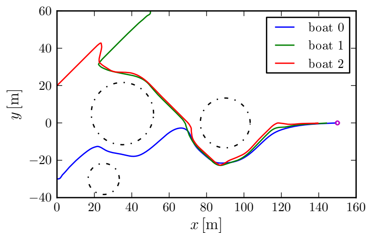
Figure 5.9: Boat trajectories
