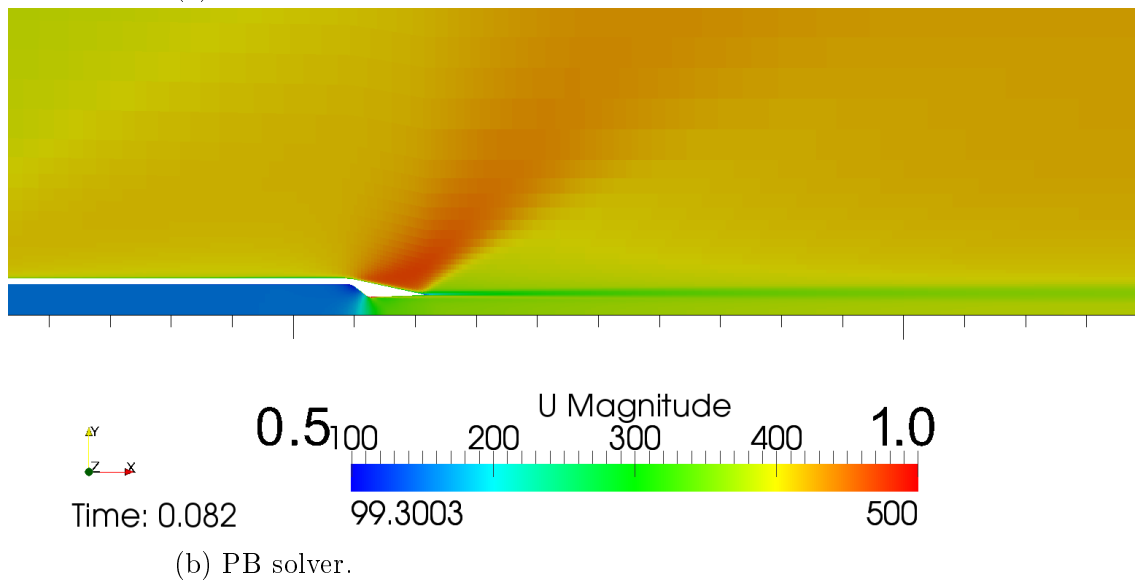
Figure 4.18: Comparison of results for different solvers with accent on shock waves on coarse level mesh, nozzle detail.
