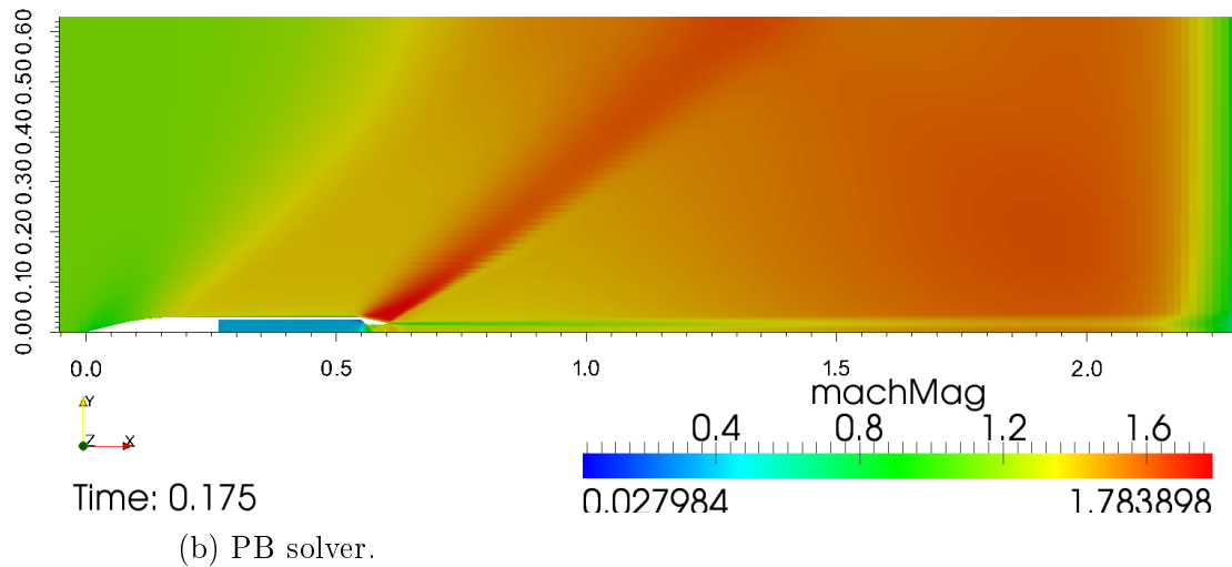
Figure 4.19: Comparison of results for different solvers with accent on shock waves on fine level mesh.
