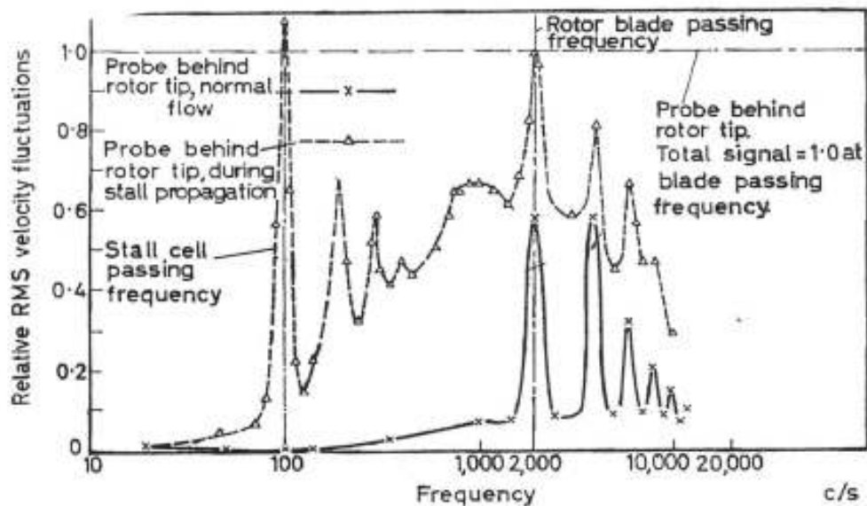
Figure 7.12. Frequencies of velocity fluctuations in compressor during rotati- stall (qualitative results only)
