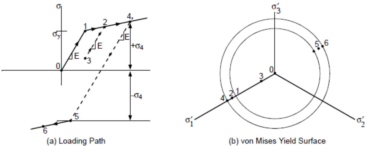
Figure 18. Isotropic hardening (3)
