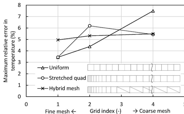
Fig. 2. Mesh sensitivity analysis of the proposed numerical method for the Stefan problem [21].
