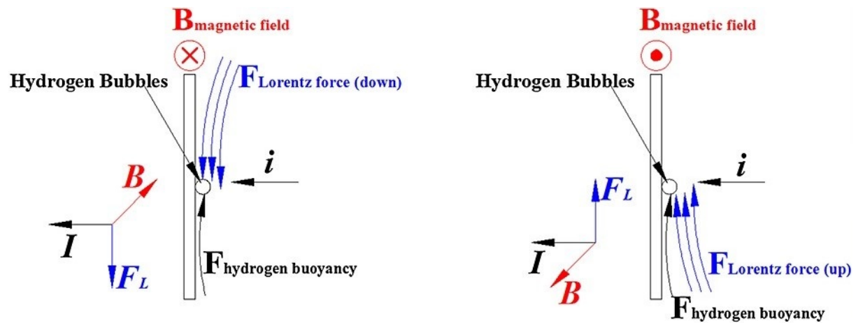
Figure 24. Differences in direction of the Lorentz force depend on the direction of the magnetic field in the relation to the direction of the electrical current [90]
