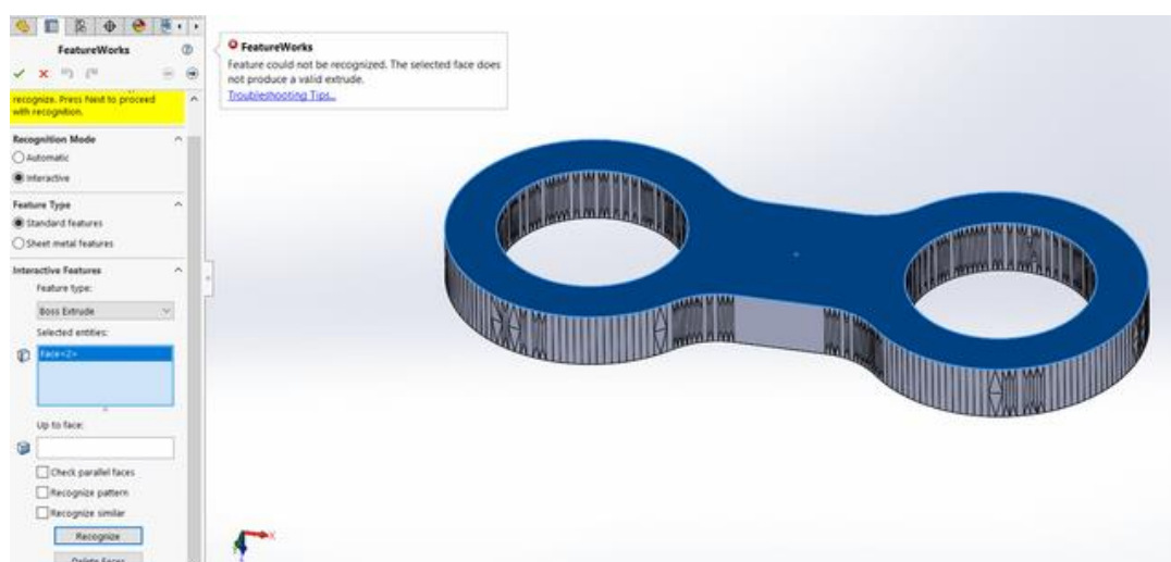
Slika 35. Solidworks FeatureWorks [58]
