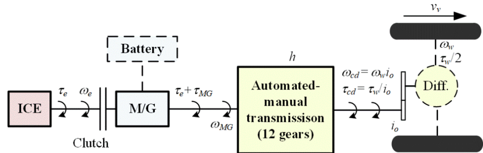
Figure 1. P2 Parallel PHEV powertrain configuration.
