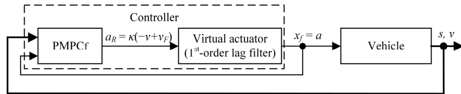
Figure 6. Block diagram of parallel MPC with virtual actuator.
