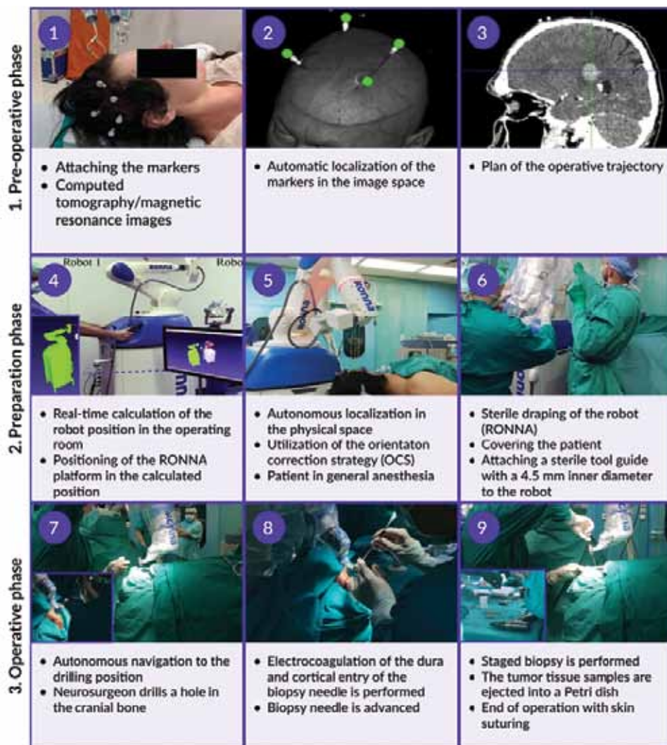
Figure 18. The application of the RONNA neurosurgical robotic system Slika 18. Primjena neurokirurškog robotskog sustava RONNA
