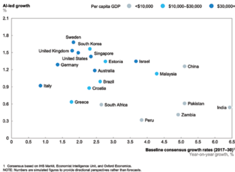
Figure 7. The adoption of artificial intelligence contributes to economic growth (Source: HIS Markit; Economist Intelligence Unit; Oxford Economics; McKinsey global institute analysis) Slika 7. Usvajanje umjetne inteligencije pridonosi ekonomskom rastu (Izvor: HIS Markit; Economist Intelligence Unit; Oxford Economics; McKinsey global institute analysis)
