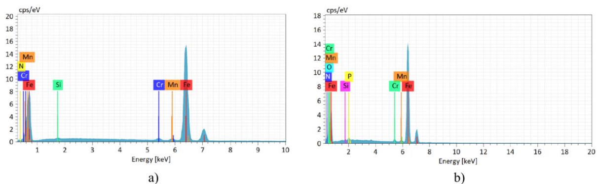
Figure 53. EDS spectrum of a) ground steel disc, b) electropolished steel disc [18]
