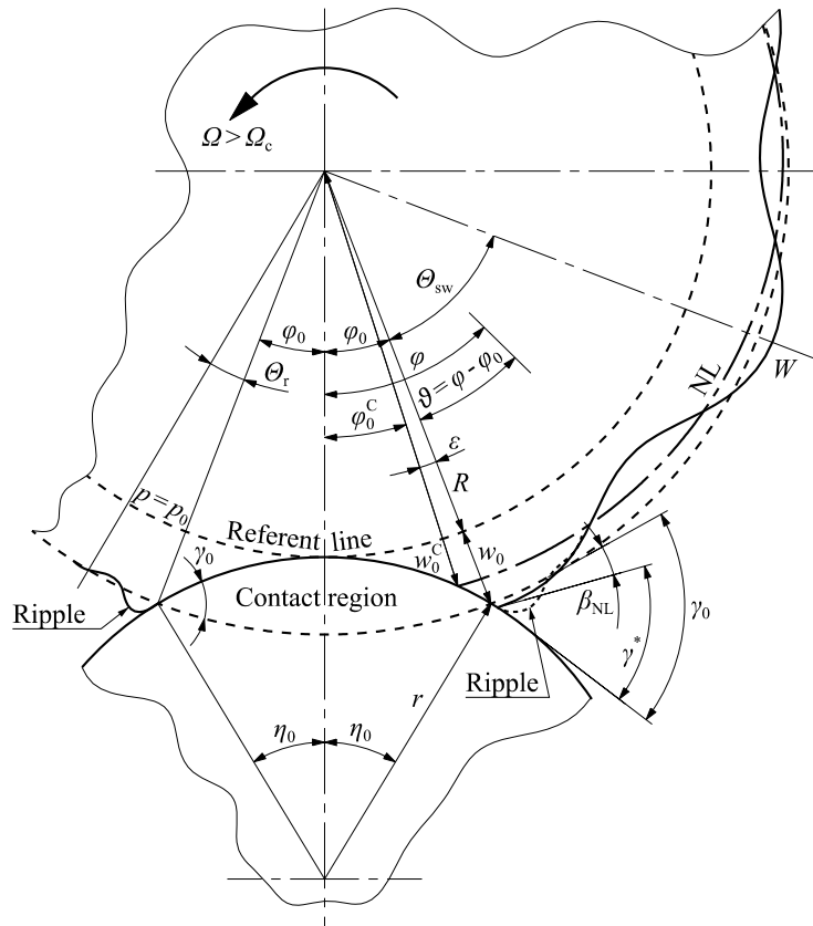
Fig. 18 Smoothing of standing waves at contact edges, boundary conditions according to experimental results, \Omega = 400 \text{ rad/s}
