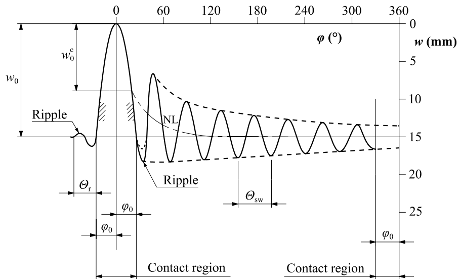
Fig. 19 Calculated ring standing waves, boundary conditions according to experimental results, \Omega = 400 \text{ rad/s}
