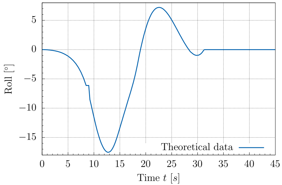
Figure 19: Prescribed roll motion.
