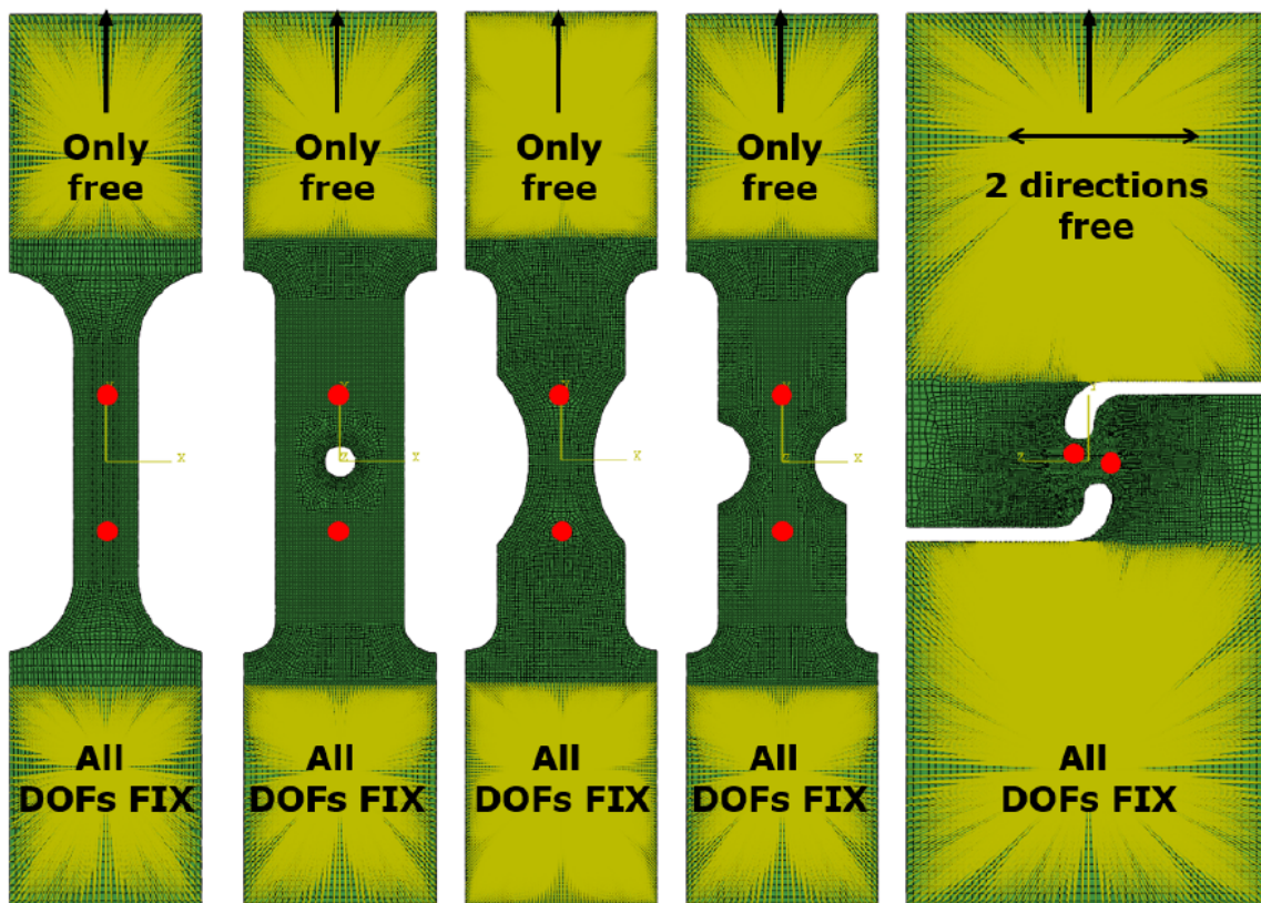
Figure 4.2: Numerical models
