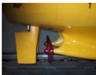
Figure 3. Twin-screw twin-skeg model.
