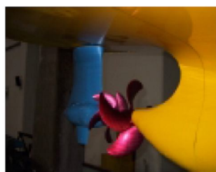
Figure 2. CRP Azipod® model.
