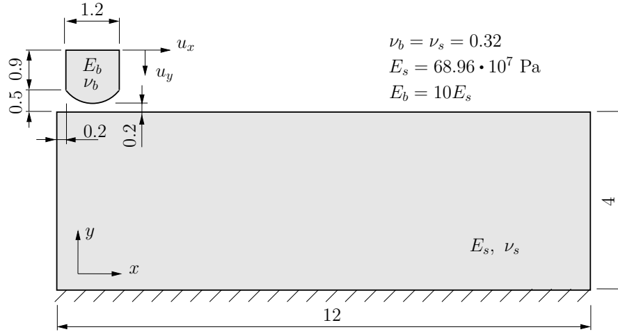
Figure 5.17. Shallow ironing: geometry description and material properties (dimensions in mm) [7]
