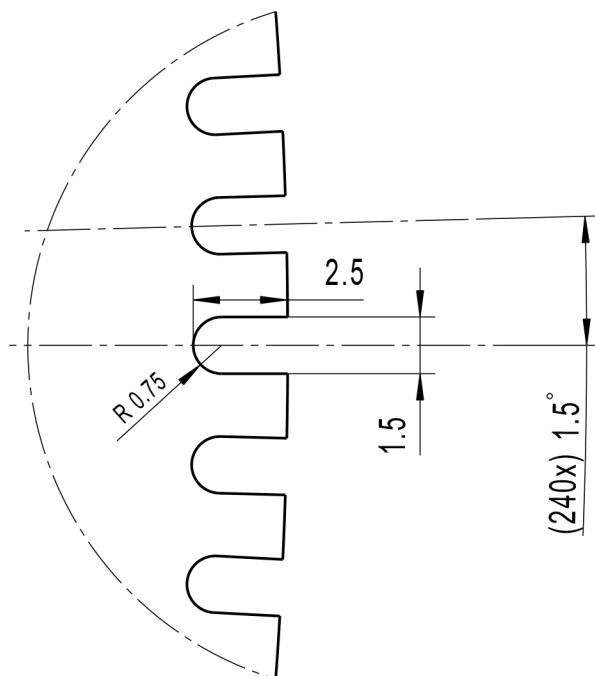
DETAIL Z (5:1)
