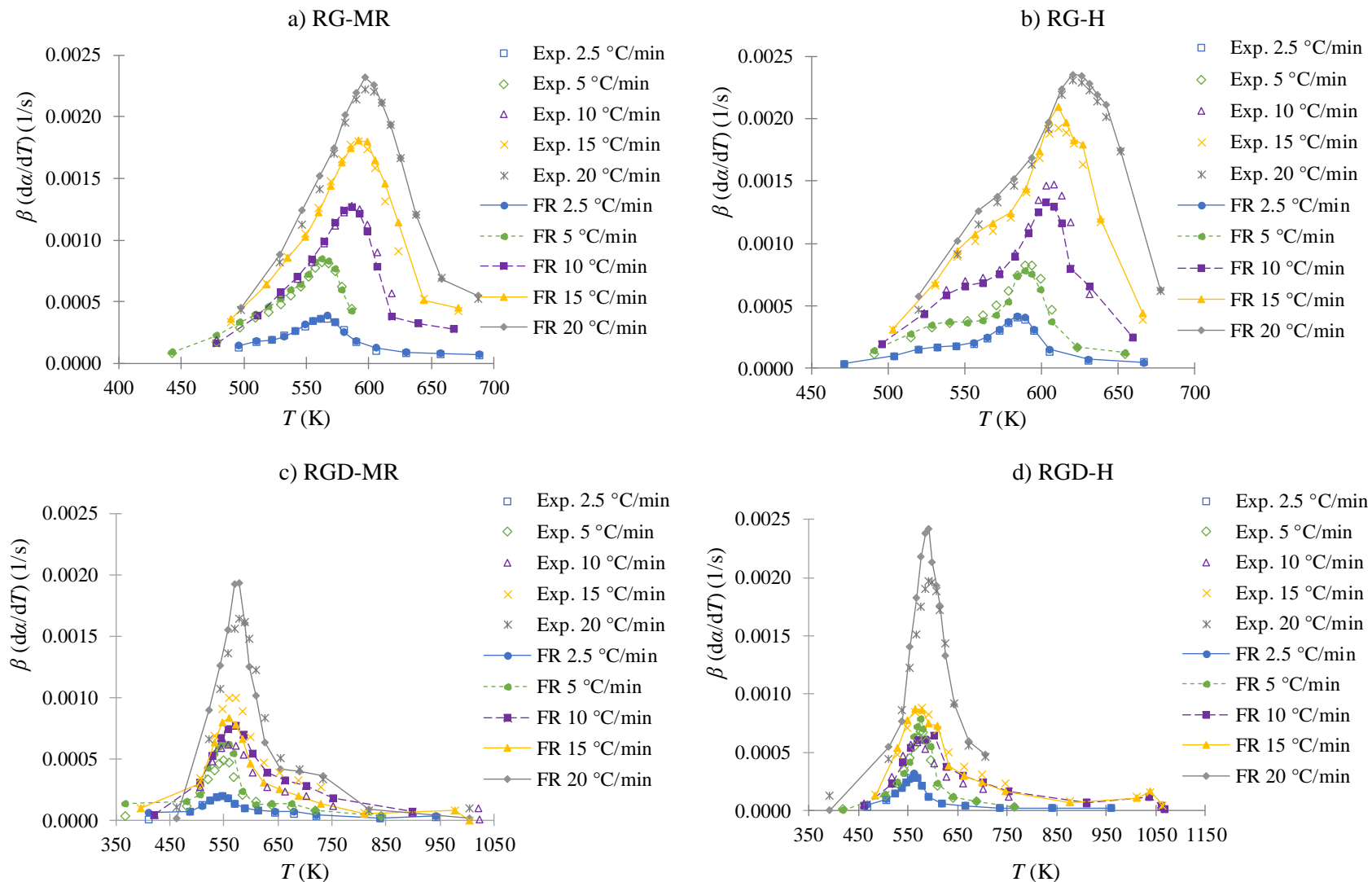
Figure 3 Experimental and FR kinetic model based on E_{\alpha} and \ln[A_{qf}(\alpha)] data for grass and digestate pyrolysis at 2.5, 5, 10, 15 and 20 ^{\circ}C/min
