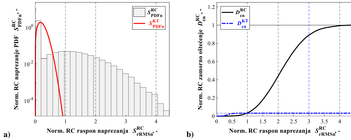
Slika 6.17 RC metoda za f_1=5\text{Hz} , f_2=100\text{Hz} , S_{\text{PSD1}}=10000\text{MPa}^2/\text{Hz} , S_{\text{PSD2}}=2,5\text{MPa}^2/\text{Hz}
