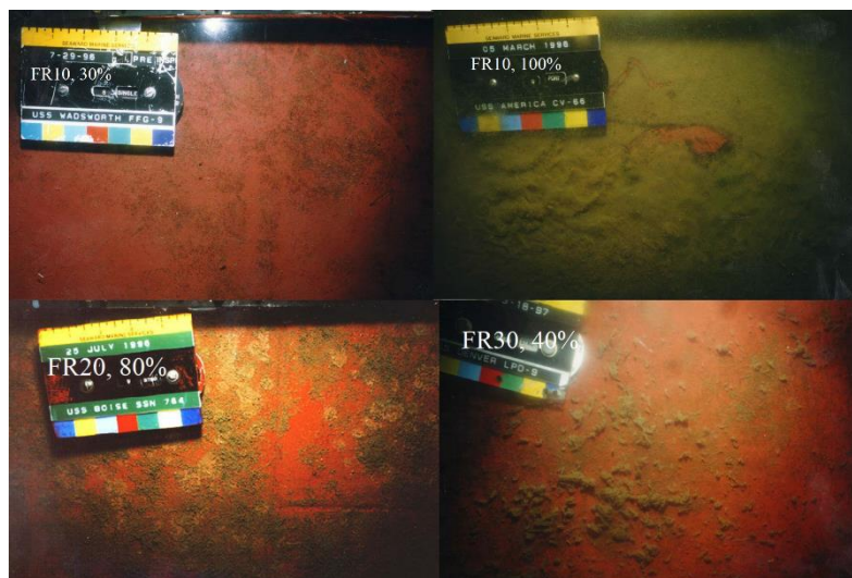
Figure 1.2 Fouling rating scale for soft fouling [40]
