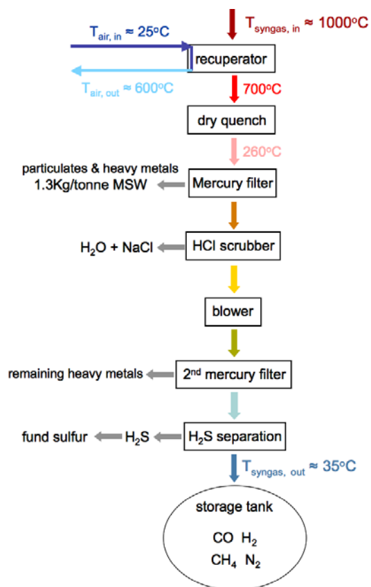
Figure 2-13: Syngas Scrubbing and Separation Flow Diagram
