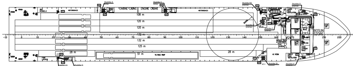
ENGINE CASING
