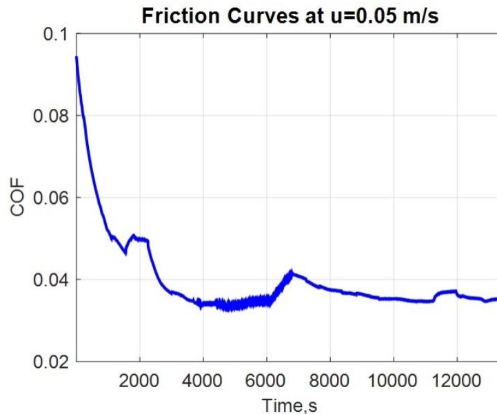
Figure 21 Diagram showing relation between COF and time [8]
